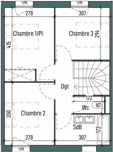
R+1
